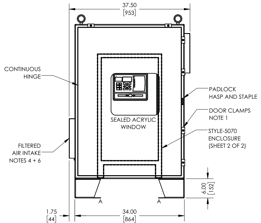
FRONT VIEW
