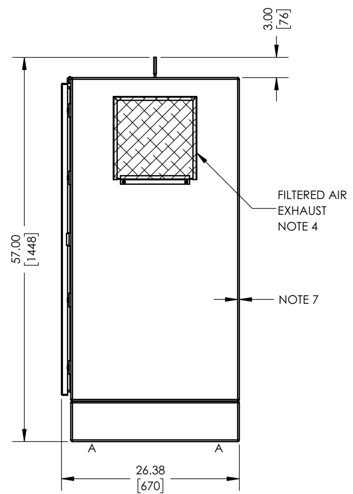
RIGHT VIEW
